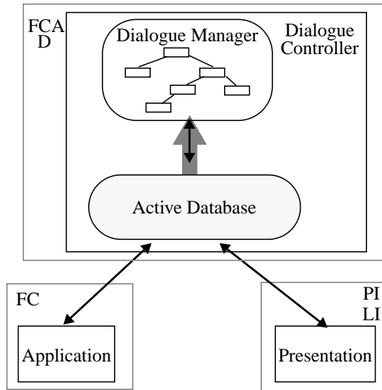
Figure 3: Serpent architecture (annotated)
