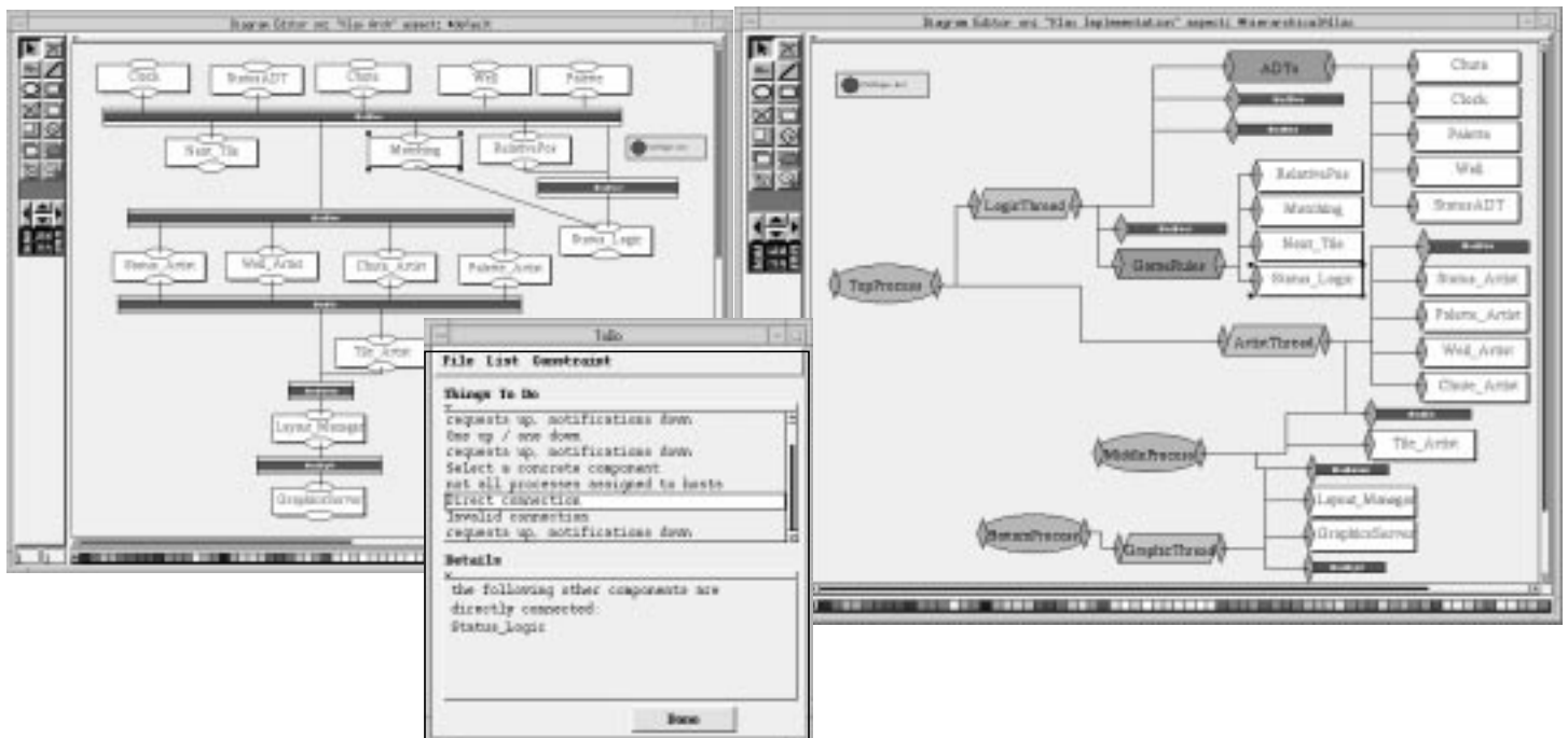
Fig. 13. Screenshots from Argo. Left: Conceptual architecture. Center: To-do list with item indicating a problem with Status_Logs. Right: Implementation Architecture. Small shapes attached to components are user interface affordances for making connections.
